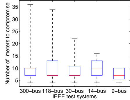
Fig. 8. Constrained case: Number of meters to compromise to inject false data into a single state variable
