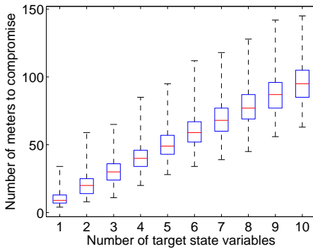
Fig. 6. Constrained case: Number of meters to compromise to inject false data into l state variables in the IEEE 118-bus system
