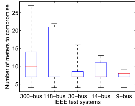
Fig. 13. Unconstrained case: Number of meters to compromise to inject false data into one state variable
