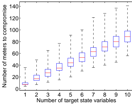
Fig. 7. Constrained case: Number of meters to compromise to inject false data into l state variables in the IEEE 300-bus system
