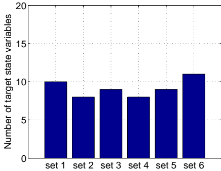
Fig. 4. Number of target state variables affected (IEEE 118-bus system)
