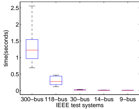
Fig. 14. Unconstrained Case: Execution time of finding an attack vector to inject false data into one state variable
