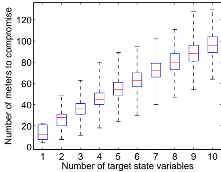
Fig. 9. Unconstrained case: Number of meters to compromise to inject false data into l state variables in the IEEE 118-bus system
