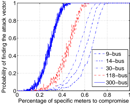
Fig. 2. Probability of finding an attack vector for random false data injection attacks
