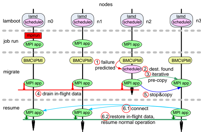
Fig. 1. Job Live Migration
