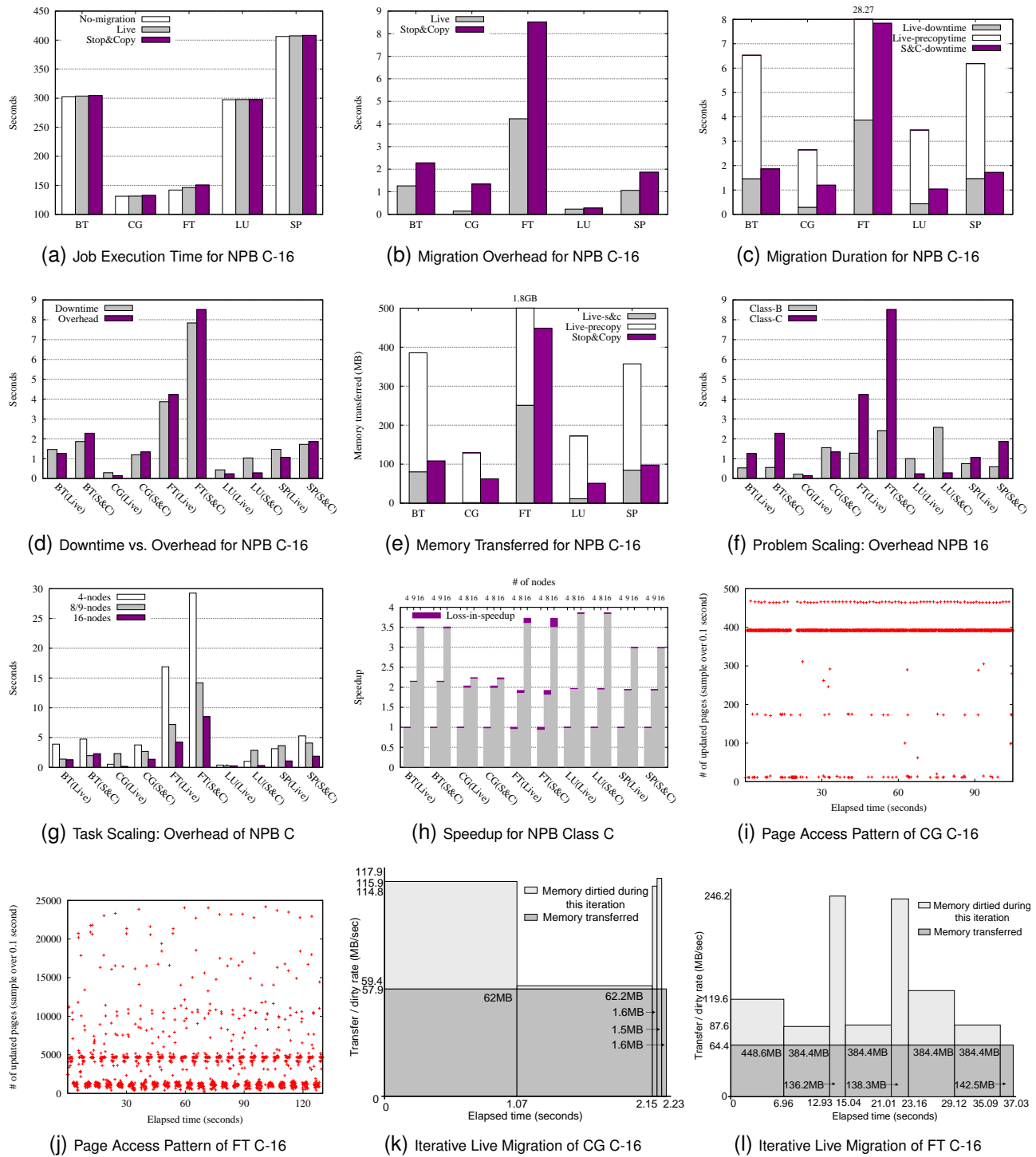
Fig. 4. Evaluation with NPB for Live Migration (C-16: Class C on 16 Nodes)
