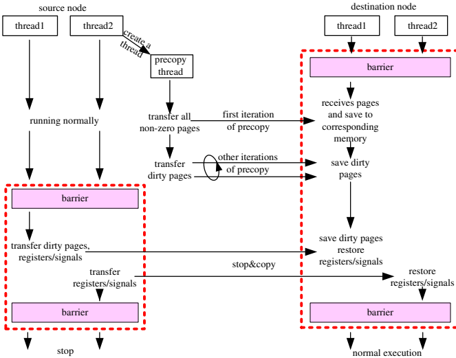
Fig. 2. Process Migration with Precopy (Kernel Mode in Dotted Frame)
