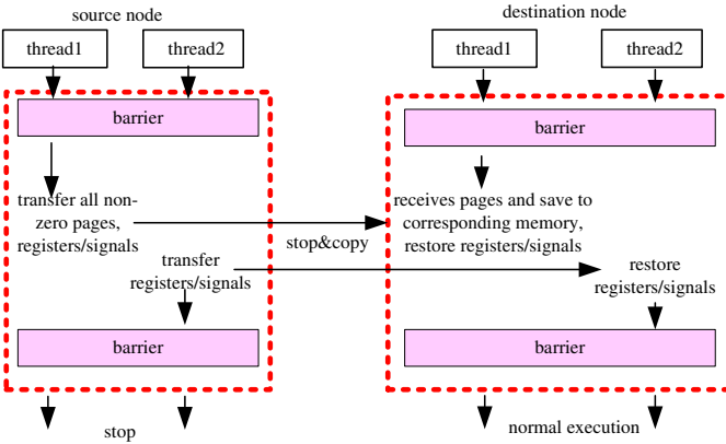
Fig. 3. Process Migration without Precopy (Kernel Mode in Dotted Frame)
