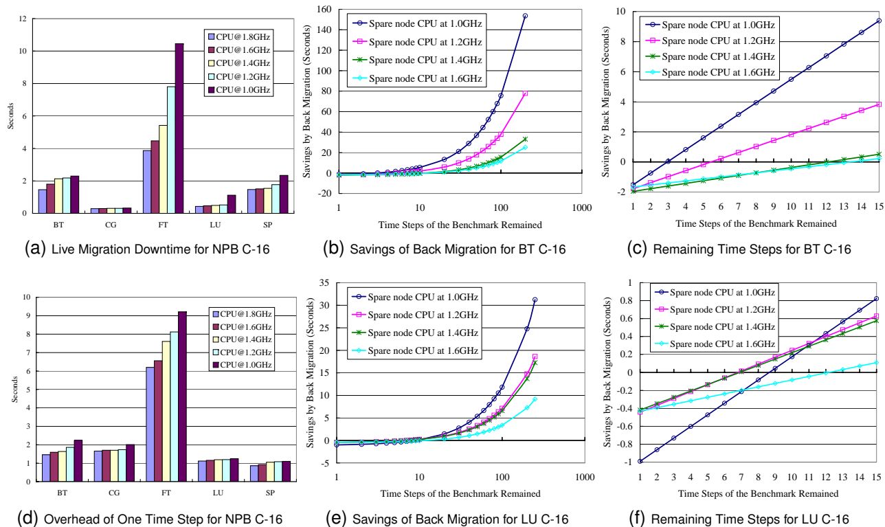
Fig. 5. NPB Results for Back Migration (C-16: Class C on 16 Nodes)
