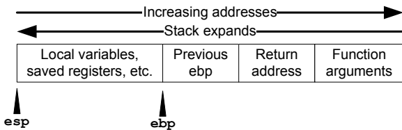
Figure 1: Simplified layout of an x86 stack frame.
