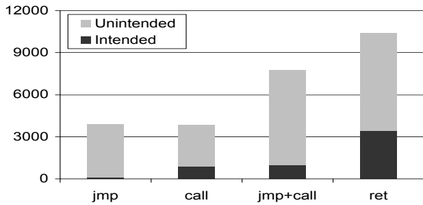
Figure 4: The frequency of indirect jmp and call instructions, both intended and unintended, vs. ret instructions in libc .
