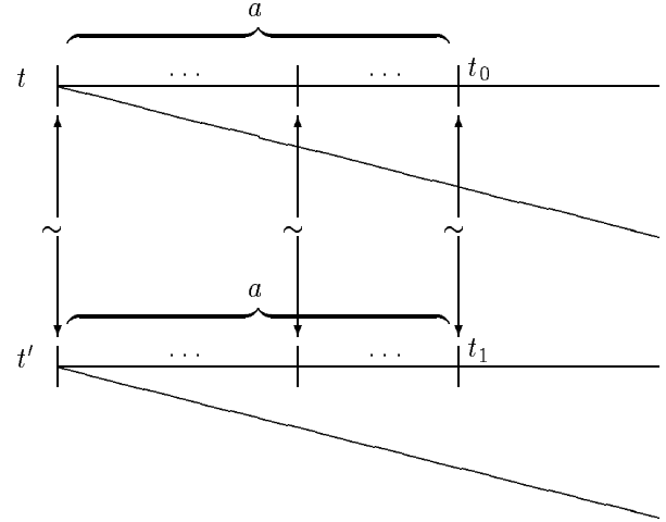
Figure 8: Weak Determinism
