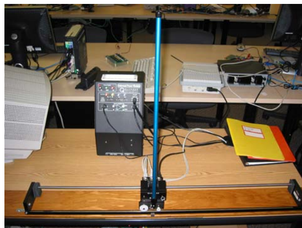
Figure 3 – Quanser System Inverted Pendulum
